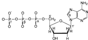
b) 2'-deoxyadenosin 5'-triphosphat (dATP) (nucleotid)
