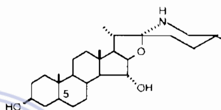
15-Hydroxysoladulcin (5 \alpha H)
