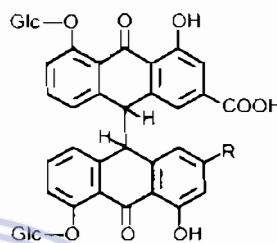
Senosid A R = COOH Senosid C R = CH 2 OH
