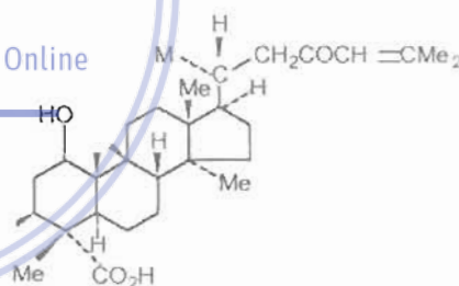
Acid gardenolic B
