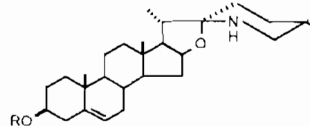
Tomatid-5-en-3 \beta -ol
