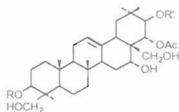
aescin
