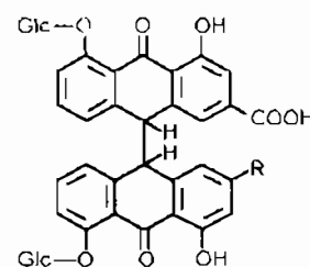
Senosid B R = COOH Senosid D R = CH 2 OH
