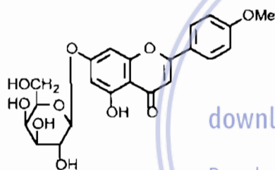
Acacetin 7-O- \beta -D-galactopyranosid
