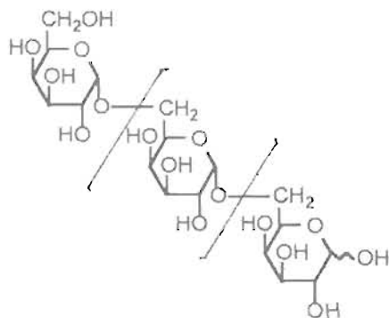
Lantanose A : x = 3
