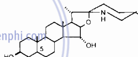
15-Hydroxytomatidin (5 \alpha H)
