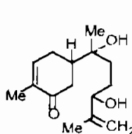
Chrysetunon
