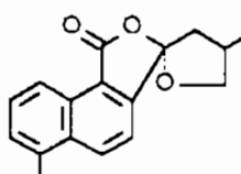
Epi - Danshenspiroketal lacton
