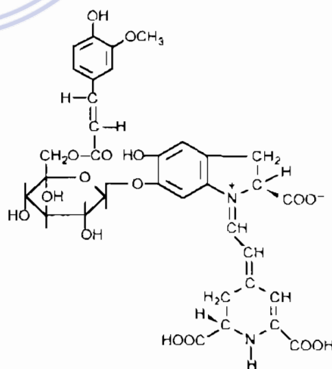
Gomphrenin - V
