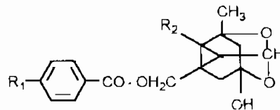
Paeoniflorin R_1 = H R_2 = \beta -glc
