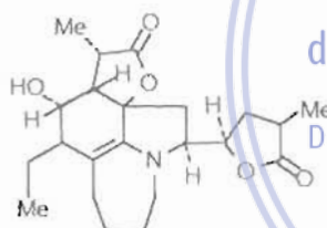
Oxotuberostemonin
