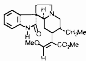
Isorhynchophyllin
