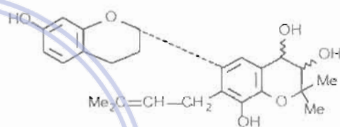
(II) Brousoflavan A
