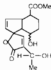
(II) \alpha OH
