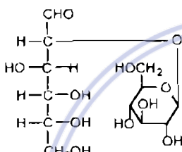
Sophorose
