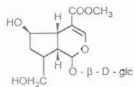
Scandosid methyl ester
