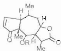
Arnicolid C : R = — CO — (CH 3 ) 2 6-O-Senecionylplenlin : R = — CO — CH = (CH 3 ) 2
