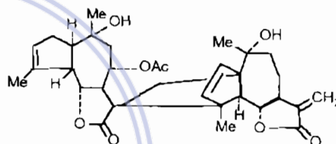
Handelin (Yejuhua lactone)
