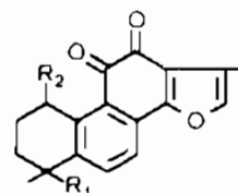
R_1 = \text{CH}_3, R_2 = \text{H}
