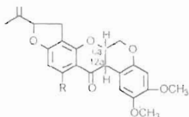
Rotenon R = H Sumatrol R = OH
