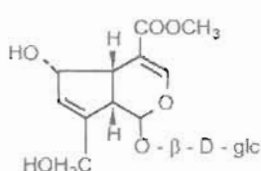
Deacetyl asperulosid methyl ester
