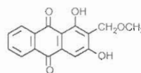
lucidin- \omega -methyl ether
