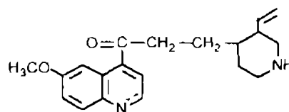
Quincin
