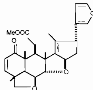
28-Deoxynimbolid
