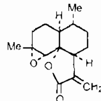
Arteannuin B (Qinghaosu II)
