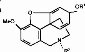
Galanthamin N-demethyl R^1 = R^2 = \text{H} Galanthamin-O-N-diacetyl R^1 = R^2 = \text{Ac}
