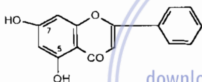
Chrysin
