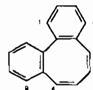
Dibenzo (a, c) cycloocten
