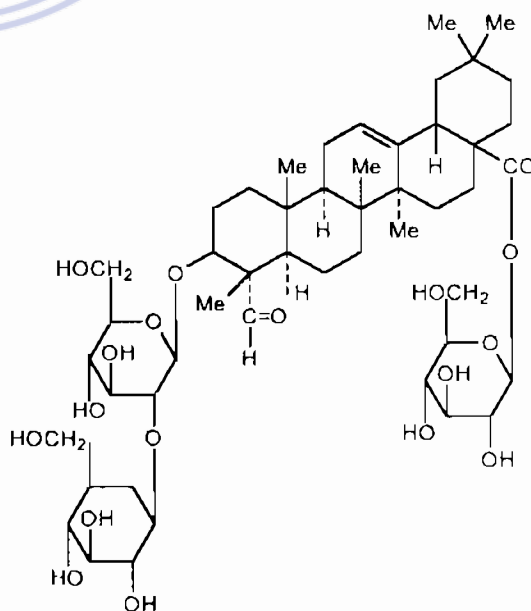
Lucycosid L 3-O- \beta -sophorosyl-gypsogenin \beta -D-glucopyranosyl ester
