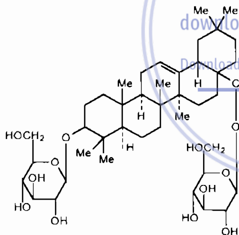
Lucycosid H 3-O- \beta -D-glucopyranosyl-oleanolic acid \beta -D-glucopyranosyl ester
