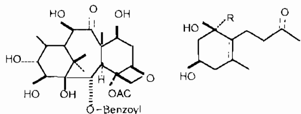
14β-Hydroxy- 10-deacetylbaccalin III
