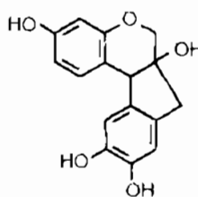
Brazilin
