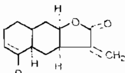
R = CHO = inulin R = CH 3 = isoalantolacton
