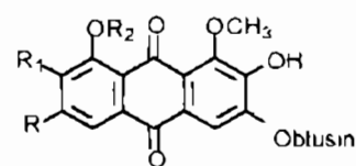
Oblusin
