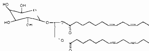
[1-O-(β galactopyranosyl)- 2-3-di-O-linolenoyl x glycerol]
