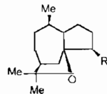
Sinenofuranal R = CHO Sinenofuranol R = CH 2 OH
