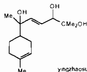
yinczhaosu D
