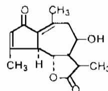
deacetyl matricarin
