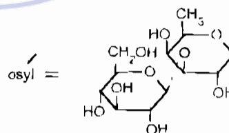
3-O- \beta -D-glucopyranosyl- \beta -D-galactopyranosyl hoặc 3-O- \beta -D-glucopyranosyl-6-deoxy- \beta -D-galactopyranosyl
