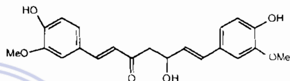
(6) dihydrocurcumin
