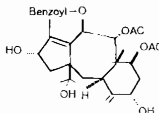
Brevifolol
