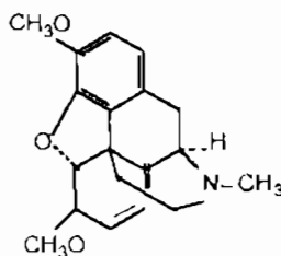
Thebain
