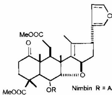
Deacetylnimbin R = H
