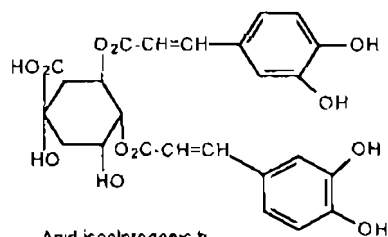
Acid isoclorogenic b
