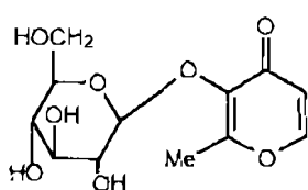
3-Hydroxy-2-methyl-pyran-4-on 3-O- \beta -D-glucopyranosid
