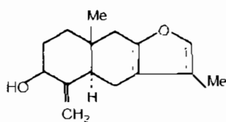
Hydroxyatractylon: R = H Acetoxyatractylon: R = AC
