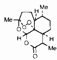
Artemisinin (Qinghaosu, Arteannuin)
