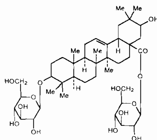
Lucycosid C 3-O- \beta -D-glucopyranosyl-machaerinic acid \beta -D-glucopyranosyl ester
