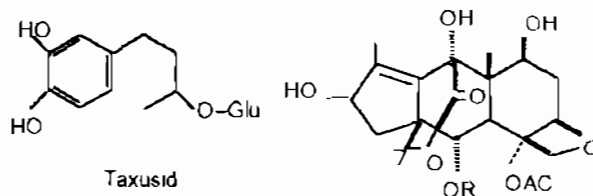
Walifolol, R = Benzoyl
