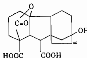
Canavalia giberellin I
