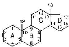
Steroid
