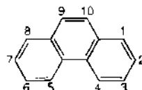
Phenanthren
