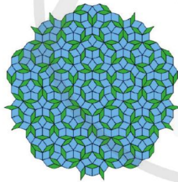
Tessellation Penrose
