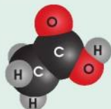
a) Acetic acid
