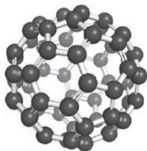
a) buckminsterfullerene
