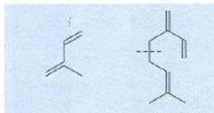
isopren, C_5H_8 limonen, C_{10}H_{16}
