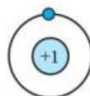
a) Hydrogen
